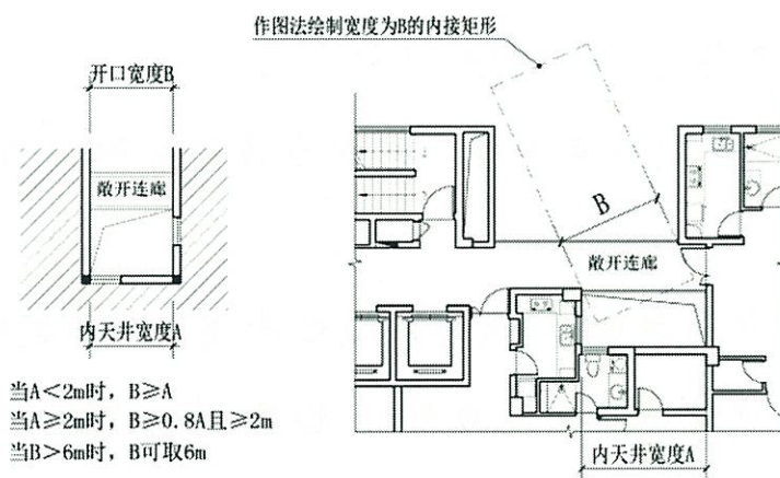
附图31: U型内天井
